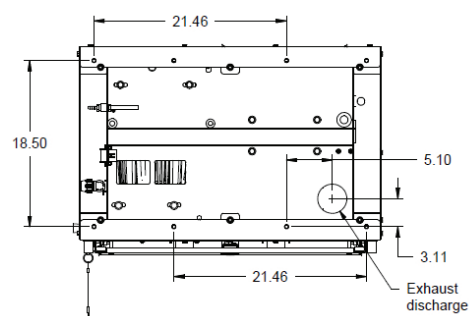
Bolt down pattern
